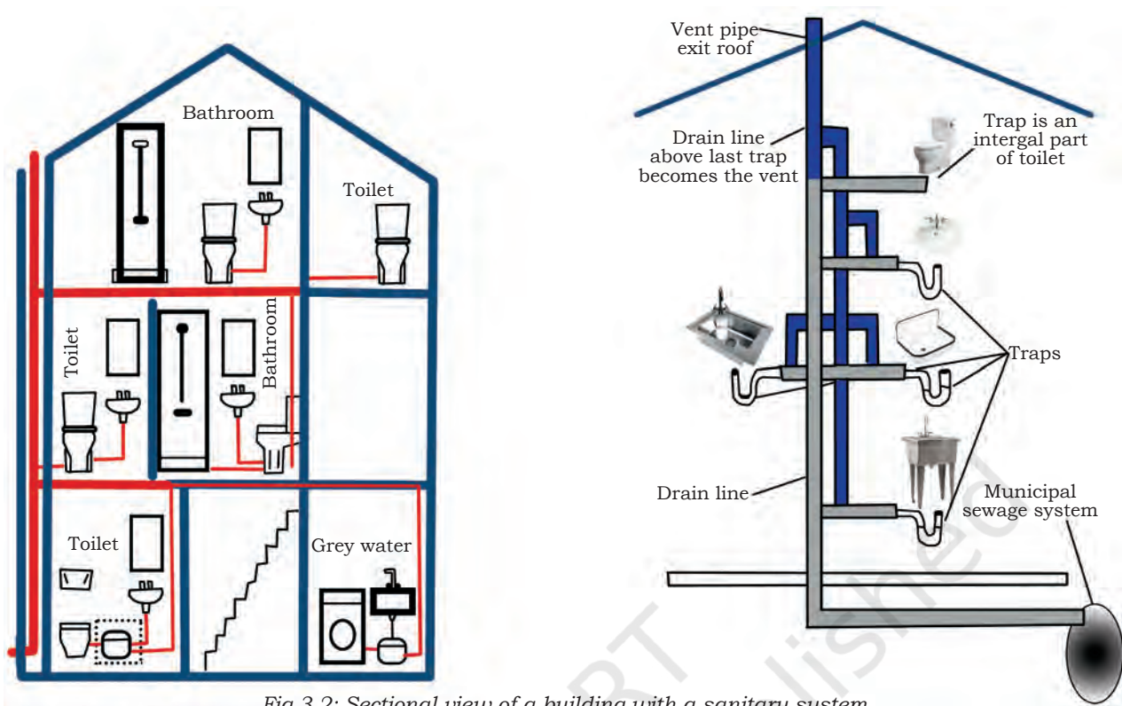
Fig.3.2: Sectional view of a building with a sanitary system
