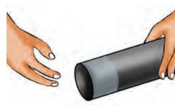
Fig.1.11: Apply the solvent on both the edges
