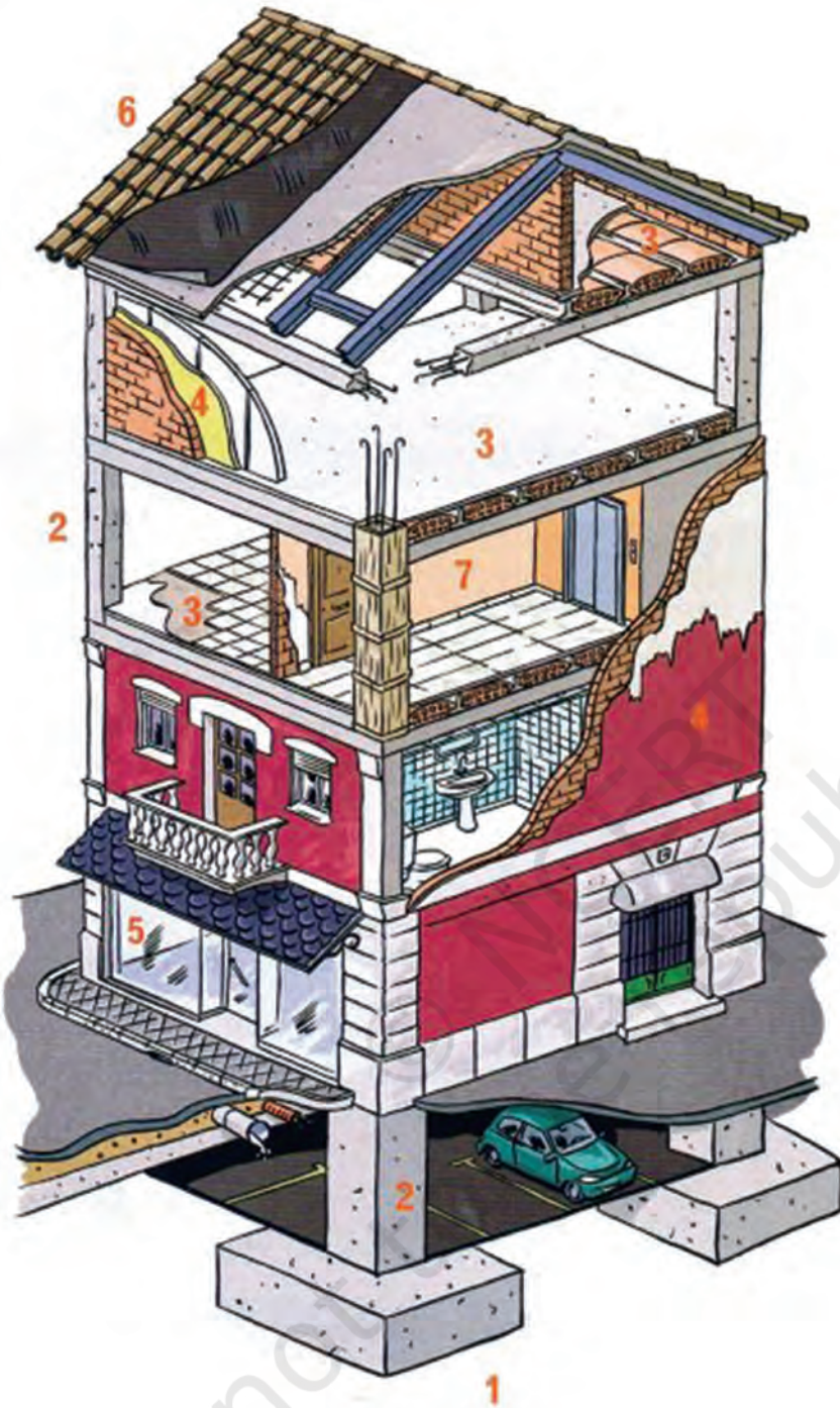
Fig.3.1: Essential elements of a modern building
